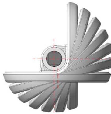
Double eccentricity
