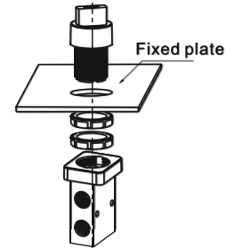
Fixation way of panel
